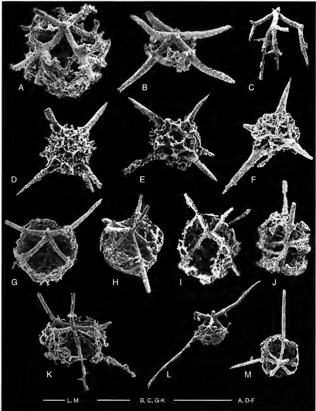
FIG. 9. — A, Parentactinia nakatsugawaensis Sashida, DEUY-YK3593; B, Parentactinia sp. A, DEUY-YK3609; C, Parentactinia okuchichibuensis (Sashida), DEUY-YK3616; D-F, Entactinia (?) tanumaensis Kamata n. sp., D, holotype, DEUY-YK3500; E, paratype, DEUY-YK3522; F, paratype, DEUY-YK3643; G-M, Parentactinia karasawayamaensis Kamata n. sp., G, paratype, DEUY-YK3654; H, holotype, DEUY-YK3495; I, paratype, DEUY-YK3653; J, over view, paratype, DEUY-YK3650; K, paratype, DEUY-YK3653; L, long apical and basal spines are preserved, paratype, DEUY-YK3657; M, over view, paratype, DEUY-YK3533. Scale bars: 100 \mu m.
